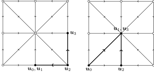
Figure 5: A path starting with the point u_0 = (1, 0, 0, 0) shown as a projection on the first two (left) and last two coordinates (right).
